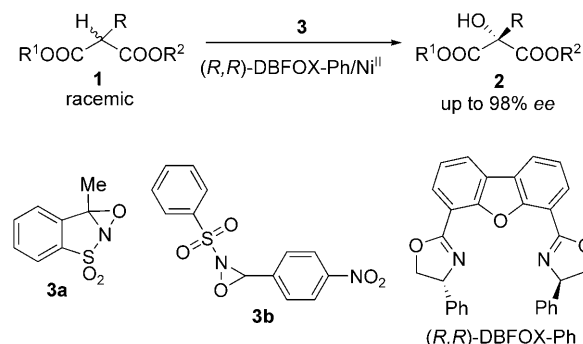
Scheme 1. A dynamic kinetic asymmetric transformation in the \alpha -hydroxylation of racemic malonate using (R,R) -DBFOX-Ph/ \text{Ni}^{\text{II}} complex with oxaziridine.
