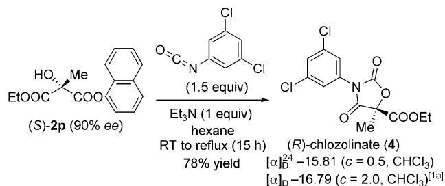
Scheme 2. Synthesis of (R) -chlozoline ( 4 ).
