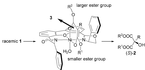
Figure 1. Transition-state structure for the (R,R) -DBFOX-Ph/ \text{Ni}^{\text{II}} -catalyzed enantioselective hydroxylation of 1 to (S) - 2 .
