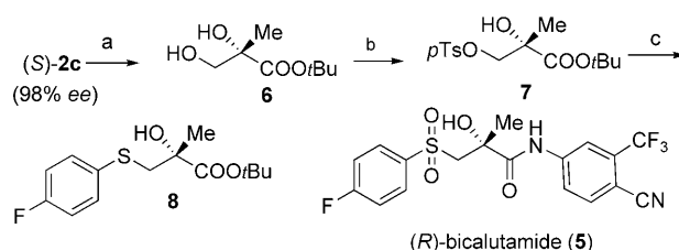
Scheme 3. Reagents and conditions: a) \text{LiAl}(\text{O}t\text{Bu})_3\text{H} (5 equiv), THF, -78^\circ\text{C} to reflux, 4 h, 66%; b) p\text{TsCl} (1.5 equiv), pyridine, \text{CHCl}_3 , 0^\circ\text{C} to RT, 17 h, 49%; c) \text{NaH} (3 equiv), 4-fluorobenzene-1-thiol (3 equiv), THF, 0^\circ\text{C} to RT, 3 h, 88%.
